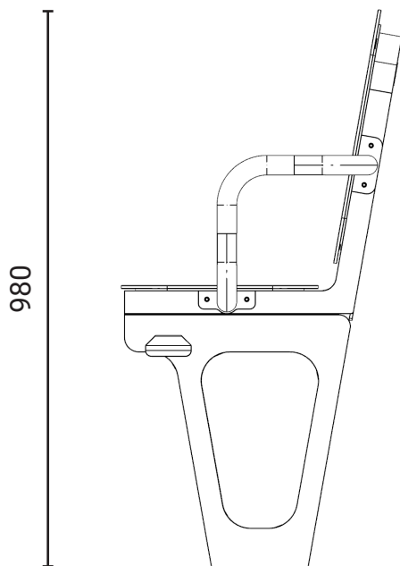
Left Elevation
