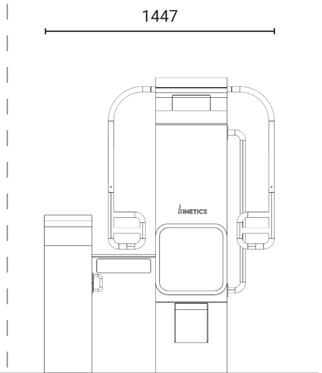
Left Elevation
