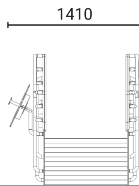
Left Elevation
