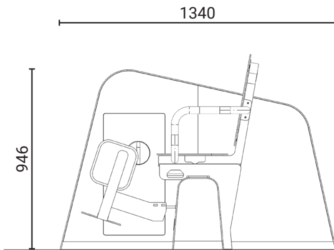
Front Elevation
