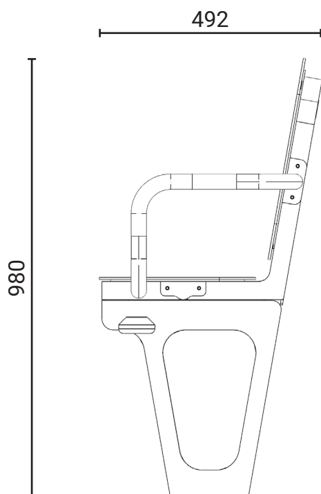
Left Elevation
