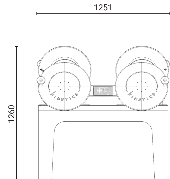
Front Elevation
