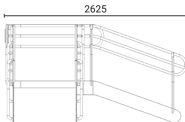
Left Elevation
